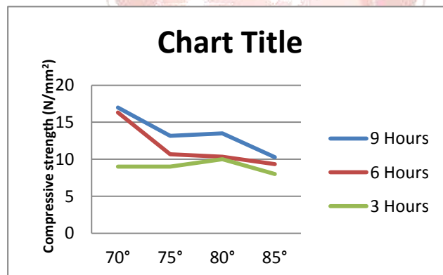
Cumulative Result based on Effect of Temperature.
