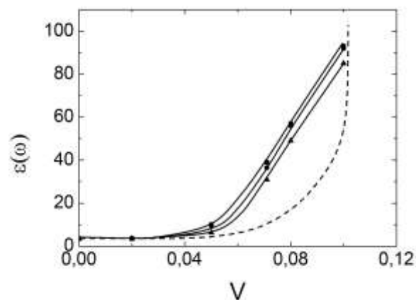
Fig. 5. V-dependences of the permittivity \varepsilon(\omega) for the metal-polymer composites containing nanoscale Ni particles. V-dependences are obtained by measurements at frequency 1000 Hz ( ) and 20 Hz ( ), by extrapolation measured data of the frequency dependences of \varepsilon to the zero frequency ( ), and by calculations in the frame of the percolation theory (the dashed line).
