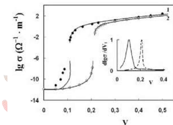
Fig. 2. Comparison of the measured (points) and calculated (solid curves) dependences of the conductivity \sigma on the fractional Ni content V for the metal-polymer composites containing nanoscale Ni particles (full points, curve 1) and micro-dispersed Ni particles (empty points, curve 2). In the insert are shown plots of the dependence of d \lg \sigma / dV on V (the solid line is for the composite containing nanoparticles, the dashed line is for the composite containing micro-dispersed particles).
