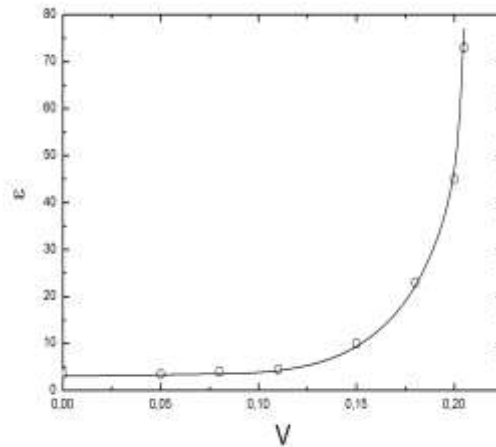
Fig. 4. V-dependences of the static permittivity \varepsilon(\omega=0) for the metal-polymer composites containing micro-dispersed Ni particles. V-dependences are obtained by calculations in the frame of the percolation theory (solid curve) and by extrapolation measured data of the frequency dependences of \varepsilon to the zero frequency (points).
