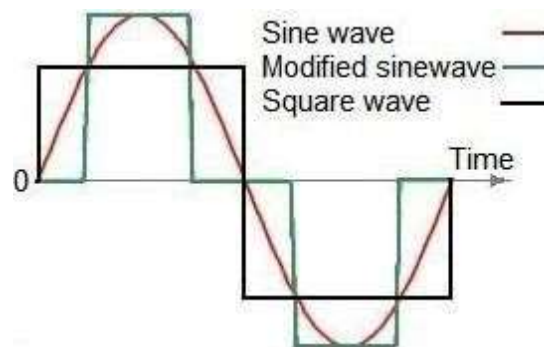
Fig. 4 Sample inverter outputs
