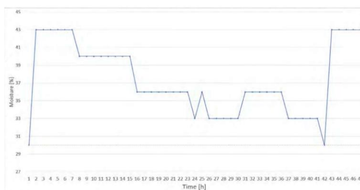
Fig: Graph showing a complete moisture level cycle
