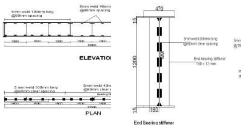
Figure 1: Details of welded plate girder of span 24 M
