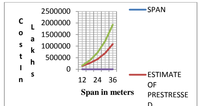
Figure 4: Variation of cost with span of girder
