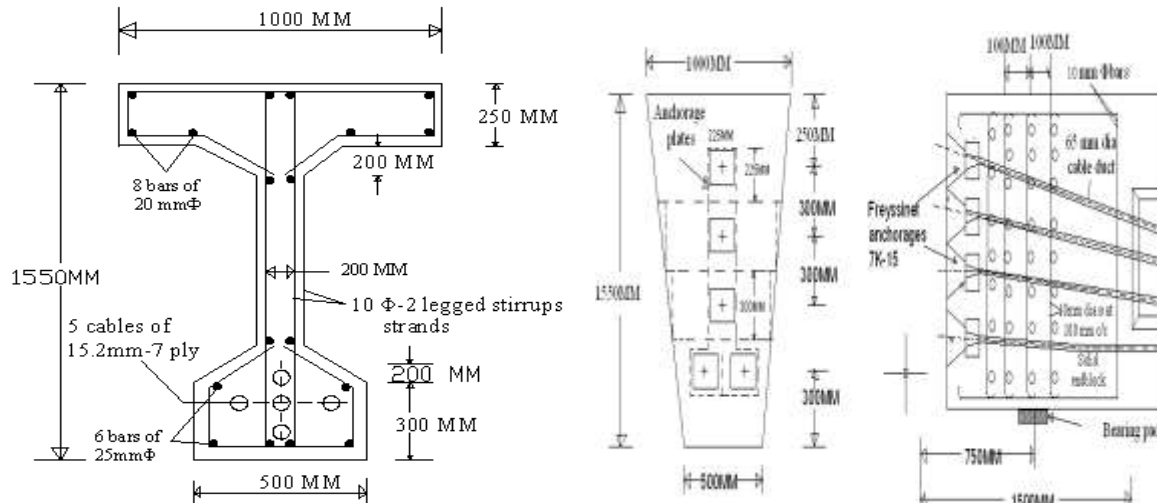
Reinforcement Details at Centre-of-Span of 24 M
