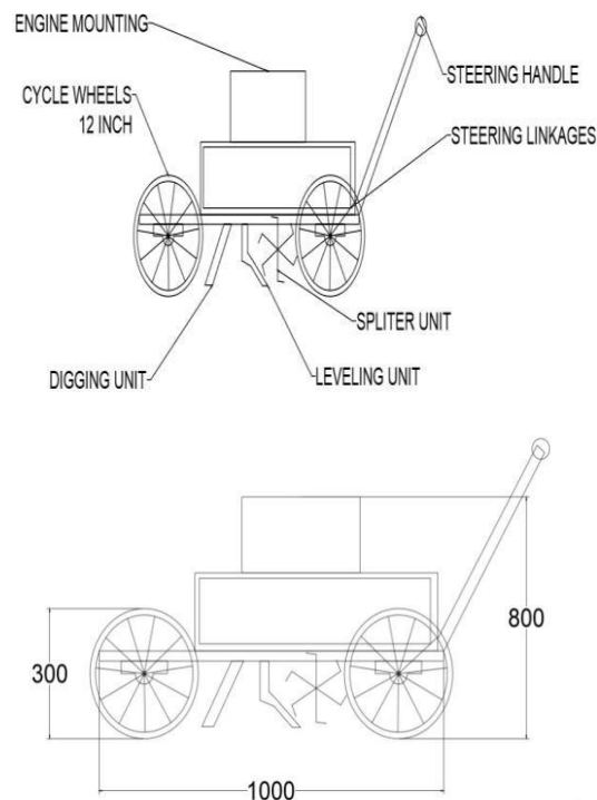
Concept diagram Multipurpose agriculture Vehicle
