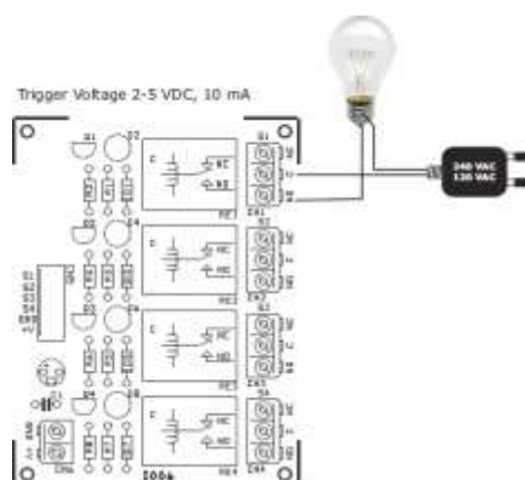
Fig -3: Relay Board Wiring Diagram
