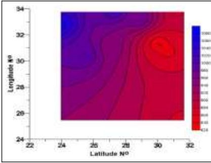
Figure 9: Output photovoltaic power from global solar radiation Wh/m 2 /day at different locations over Egypt.
