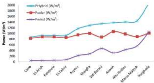
Figure 12: The hybrid energy of solar and wind for different regions over Egypt.
