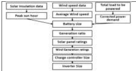
Figure 3: Flow chart of hybrid solar-wind resource.
