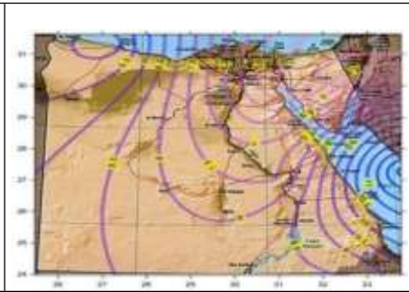
Figure 8: Annual mean of wind speed (km/h) at different locations over Egypt.
