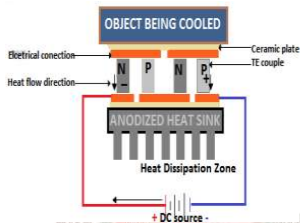
Figure 2: Working of Peltier Device System assembly:
