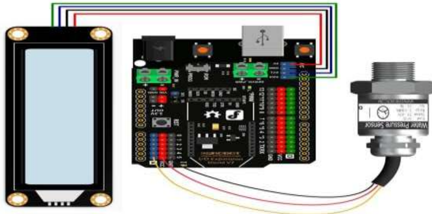
Figure 4. Wiring diagram of I2C LCD display and PSI Pressure sensor with Arduino device
